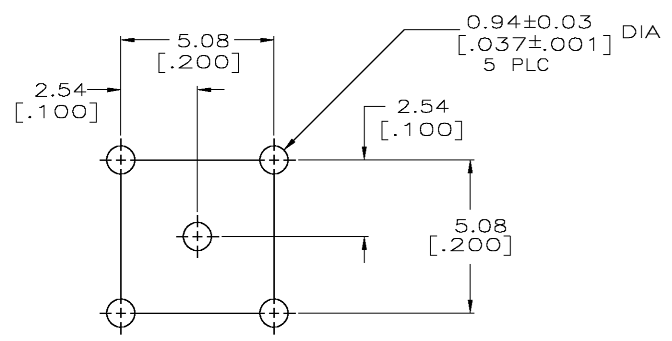
PCB CONFIGURATION
